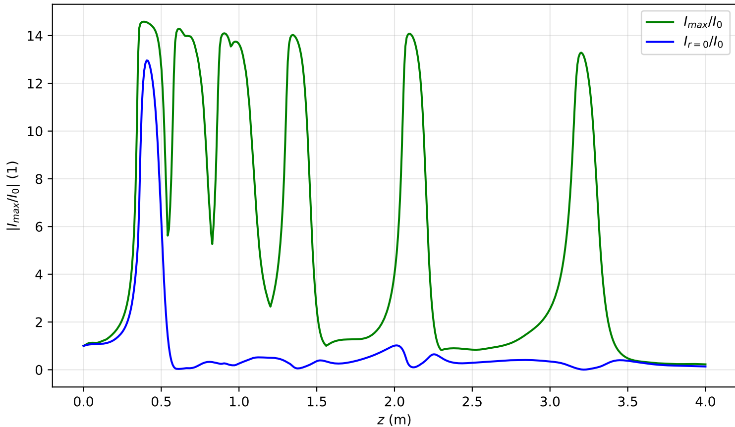
I_{max}(x=0, y=0, z)/I_0 , P_{in}=7.6P_{cr} , noisy input, artificial time
